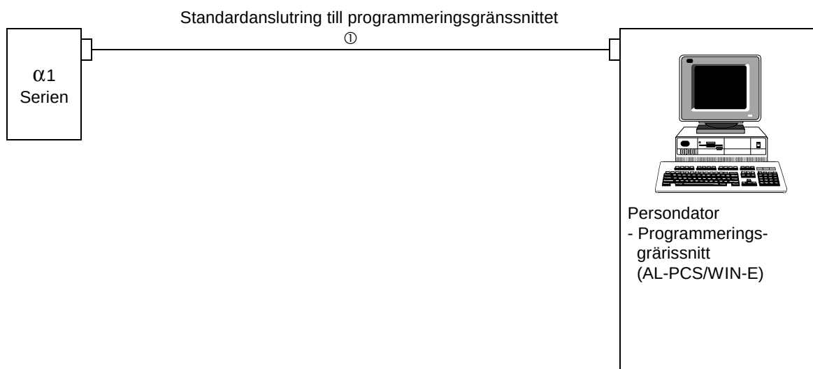
Figur 1.3: Systemkonfiguration(AL2-10MR-*)
