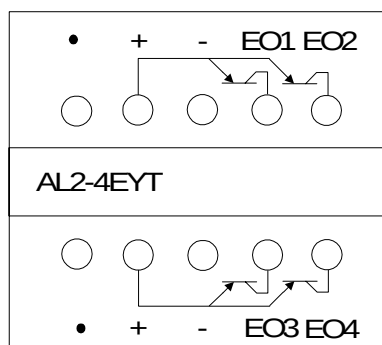
Figure 5.10: AL2-4EYT, Transistor Output
