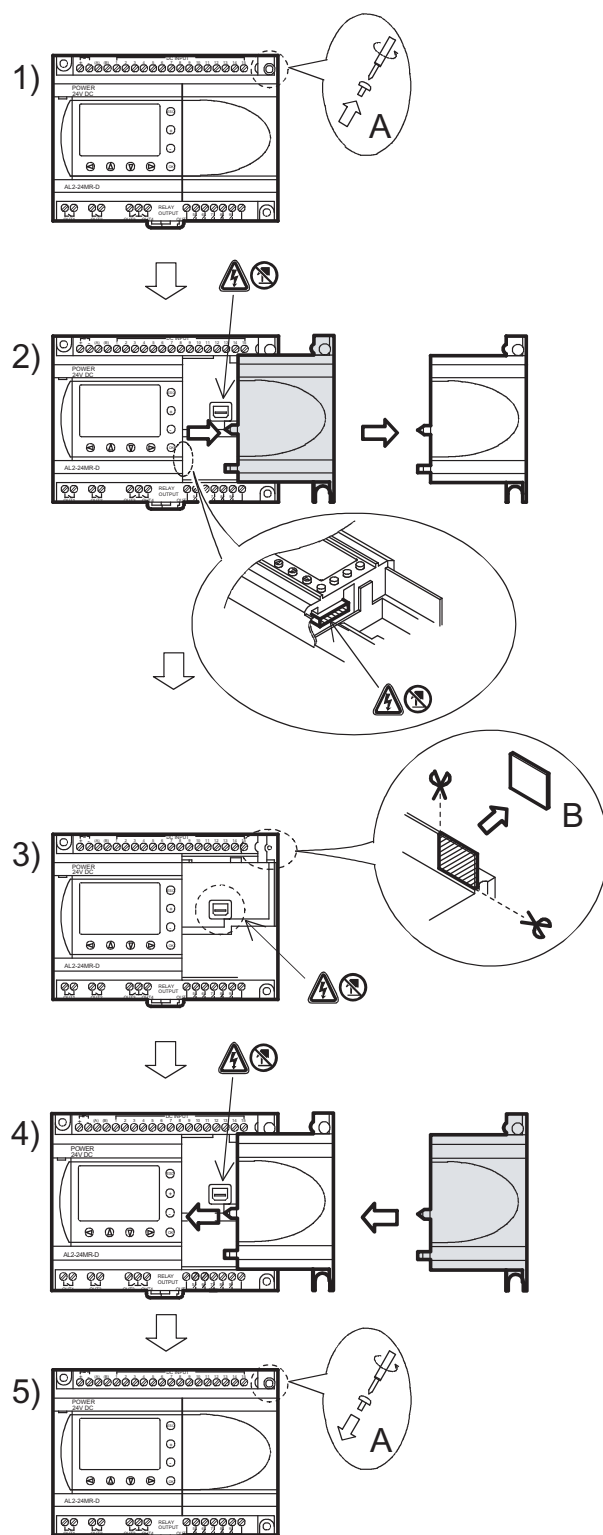
Figure 3.5: Installation
